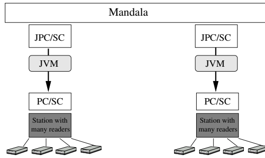
Fig. 3. The software framework.
