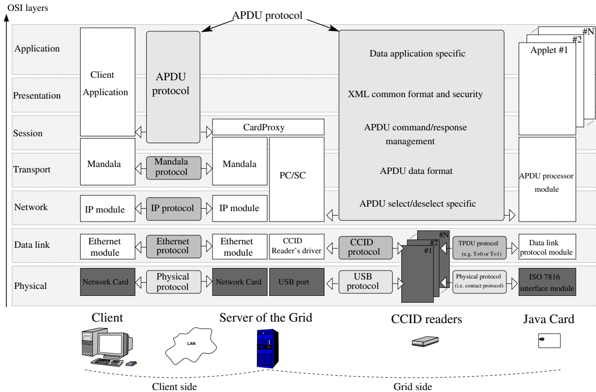
Fig. 4. Communication stack.
