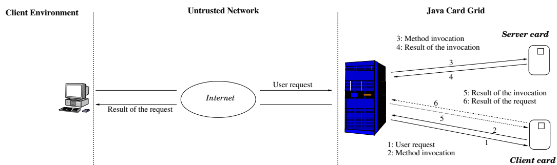
Fig. 6. Remote method invocation between cards.
