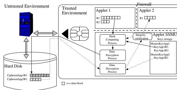
Fig. 7. Overview of the SSMU architecture.
